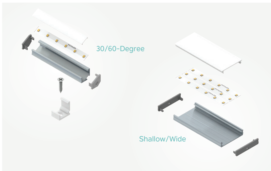
EXPLODED VIEW
